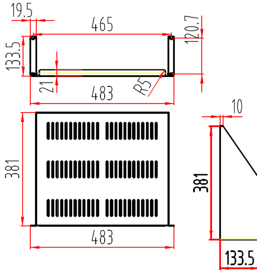
3U15" VENTED SHELF, SINGLE SIDE
