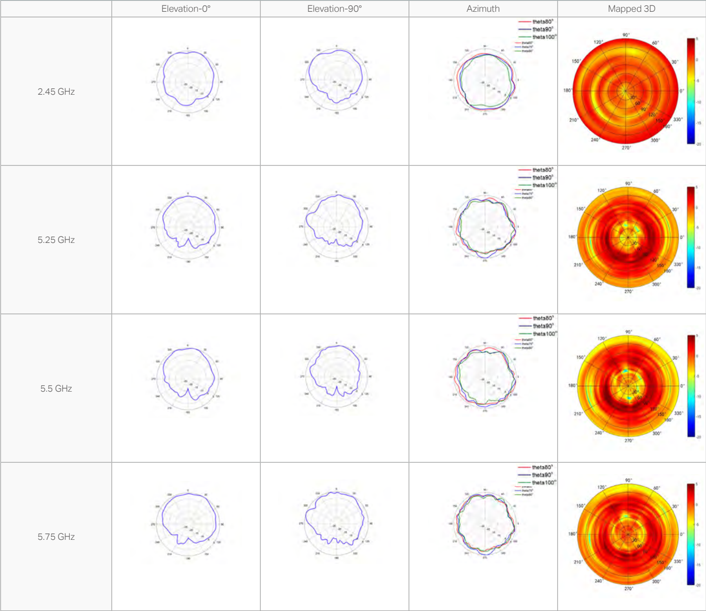
EAP650-Outdoor
