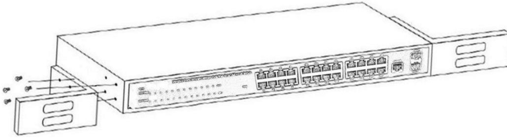
Figure 5 - Bracket Installation
