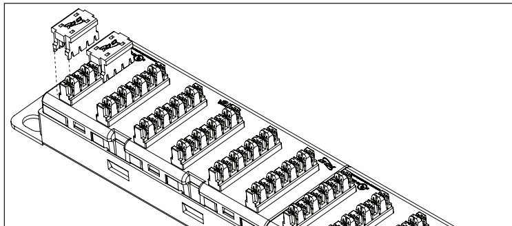
Optional. Install retention cap on 110-Type IDC to secure terminated wires. Part No. IC110TC450
