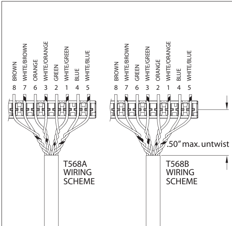
Step 1. Choose between T568A or T568B wiring configuration.
