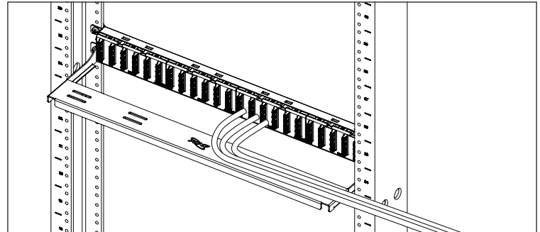
Optional. Install 5" deep cable management bar on the rear of the patch panel. Part No. ICCMSRCMRP (Recommended)
