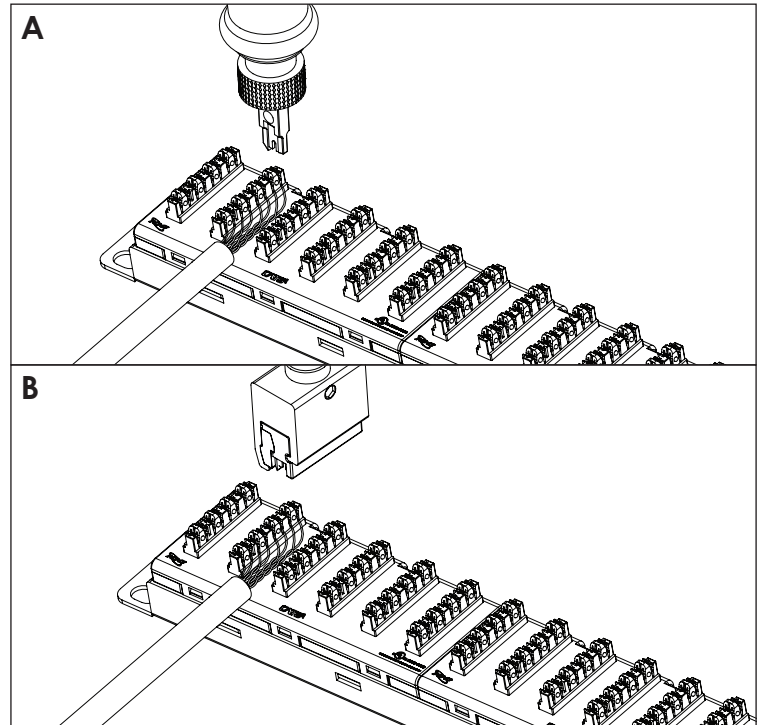
Step 2. Terminate conductors using a single blade punch down tool (A) or a four pair punch down tool (B).
