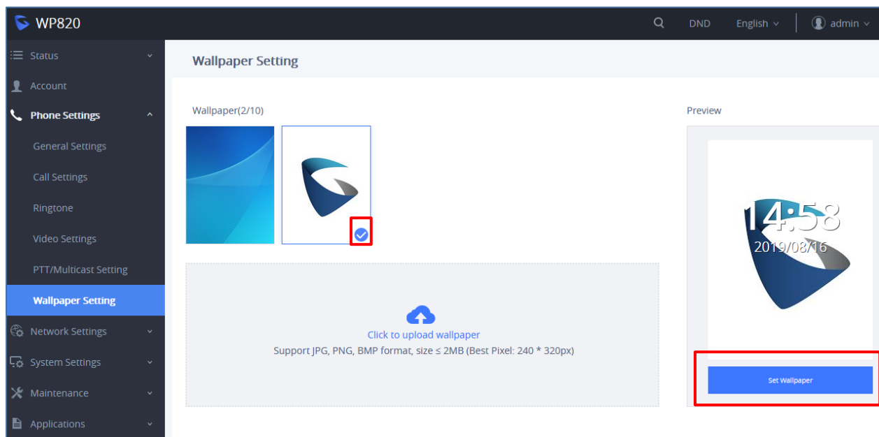
Figure 44: Switching Wallpaper from Web GUI
