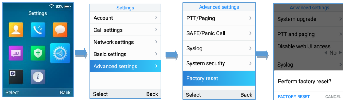
Figure 98: WP820 LCD - Confirm Factory Reset
