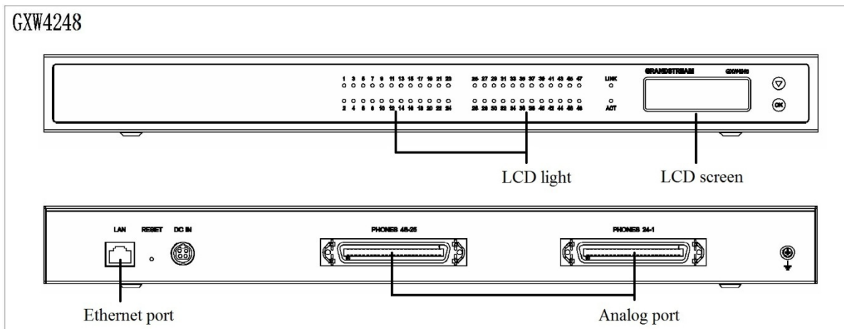
FIGURE 1: DIAGRAM OF GXW4216/24/32/48 PANEL
