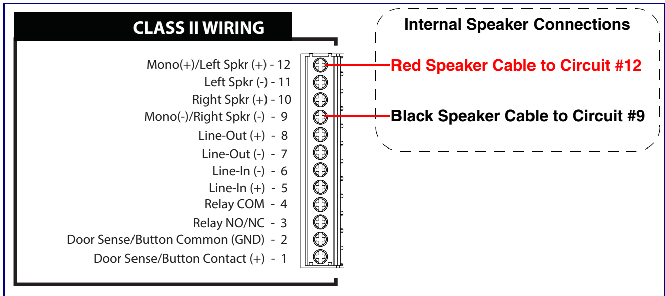
Figure 2-4. Singlewire InformaCast IP66 Outdoor Horn Connections
