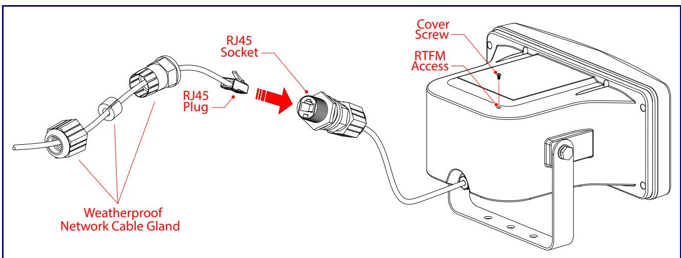
Figure 2-5. Install the Network Cable Through Weatherproof Cable Gland
