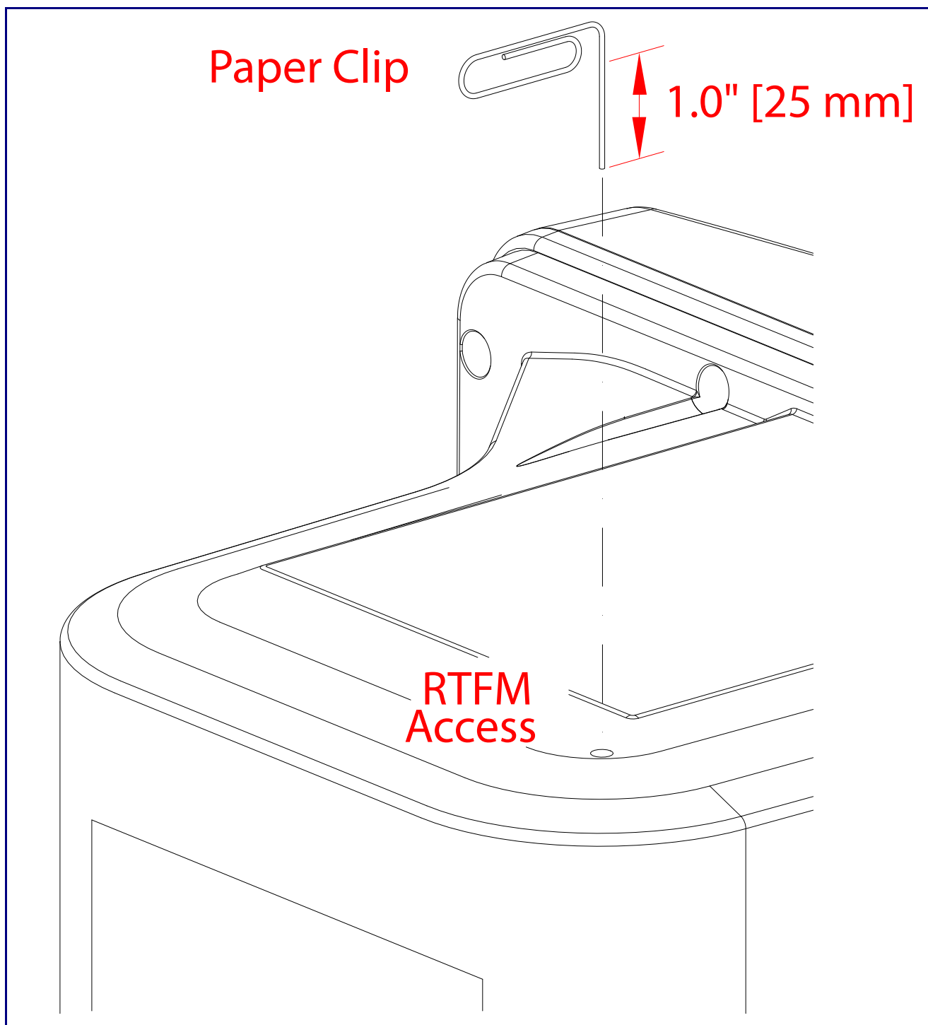
Figure 2-8. RTFM Switch
