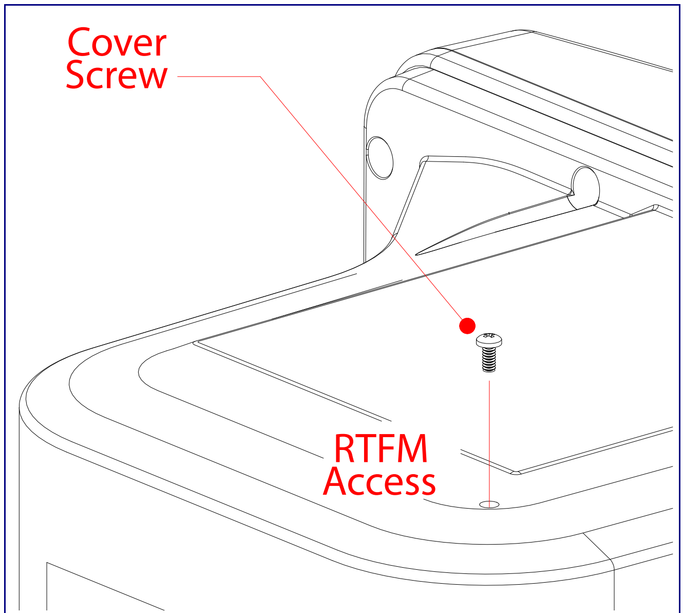
Figure 2-7. RTFM Switch
