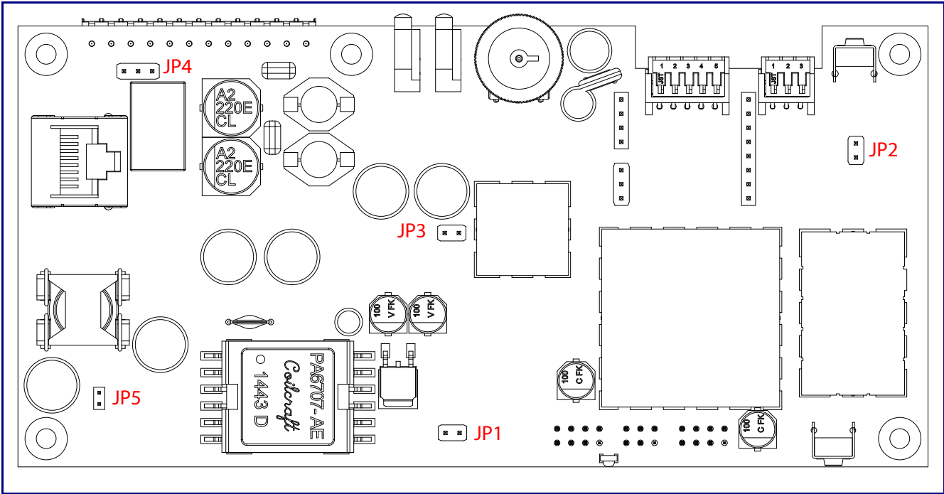
Figure 2-14. Jumper Locations
