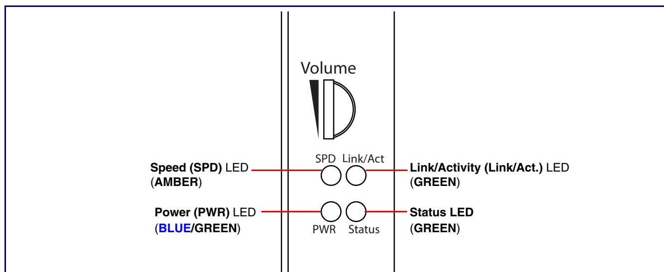
Figure 2-16. SIP Loudspeaker Amplifier (PoE) LEDs
