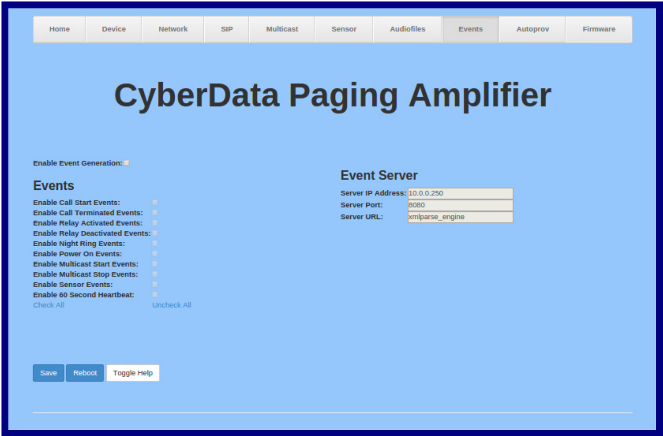
Figure 2-37. Event Configuration Page
