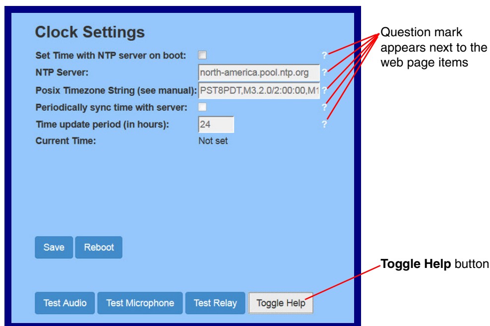
Figure 2-21. Toggle Help Button and Question Marks
