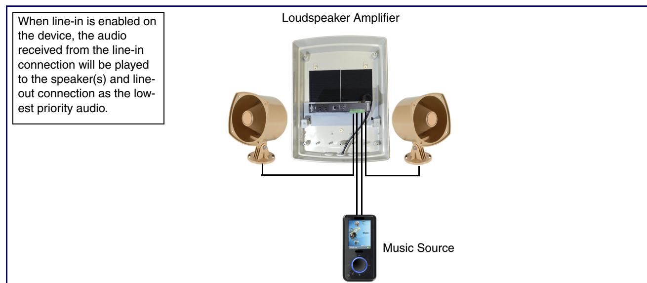
Figure 2-10. Line-In Connection
