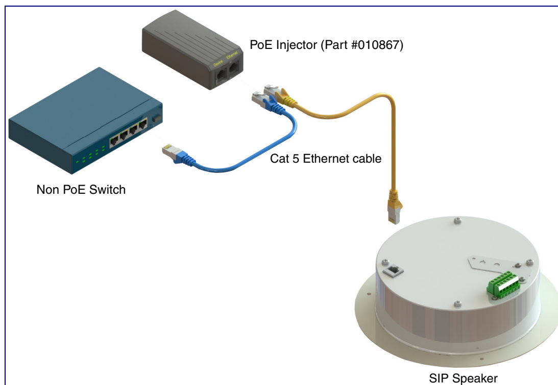
Figure 2-2. SIP Speaker (with PoE Injector) to a Non PoE Switch
