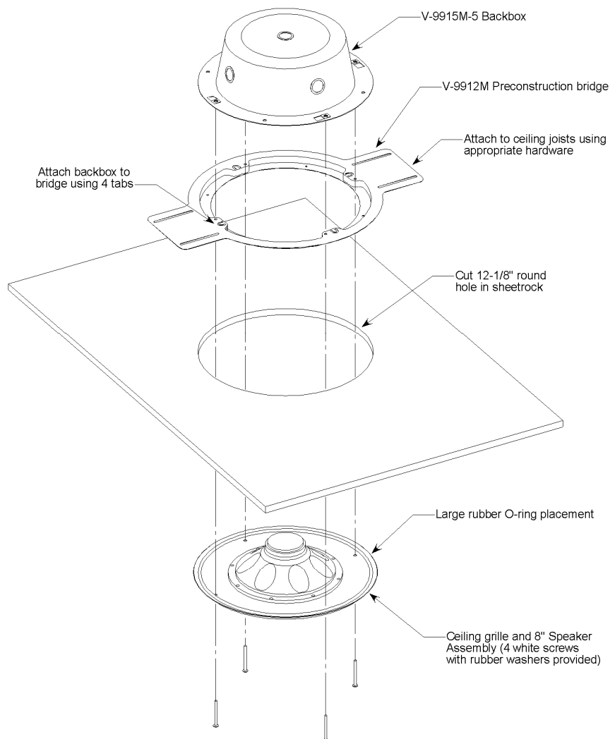
FIGURE 3: V-1040 INSTALLATION INSTRUCTIONS HARD CEILING
