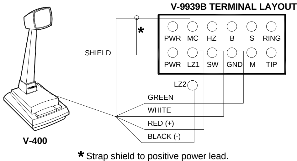
FIGURE 1 - CONNECTING ARRANGEMENT
