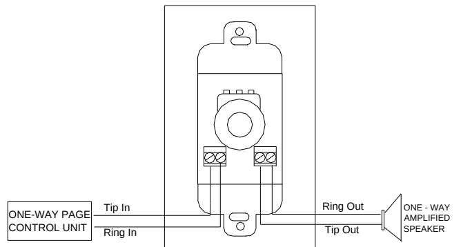
V-2992 CONNECTIONS USING A ONE - WAY PAGE CONTROL
