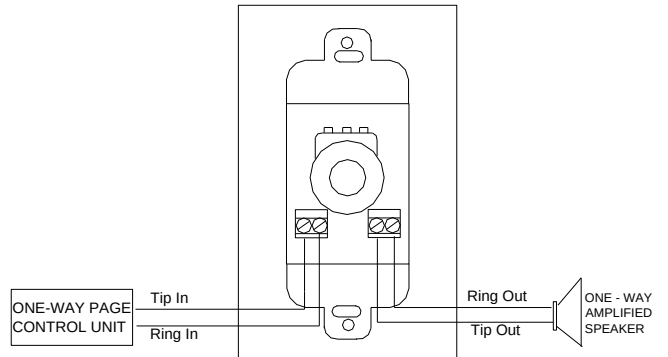
V-2992 CONNECTIONS USING A ONE - WAY PAGE CONTROL
