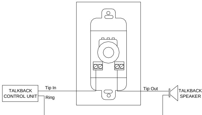
V-2992 CONNECTIONS USING A TALKBACK PAGE CONTROL
