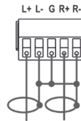
Figure 6: Connecting an Unbalanced Stereo Audio Source to the Balanced Input
