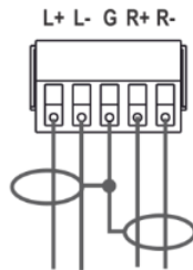
Figure 5: Connecting a Balanced Stereo Audio Source to the Balanced Input
