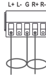
Figure 4: Connecting to an Unbalanced Stereo Audio Acceptor
