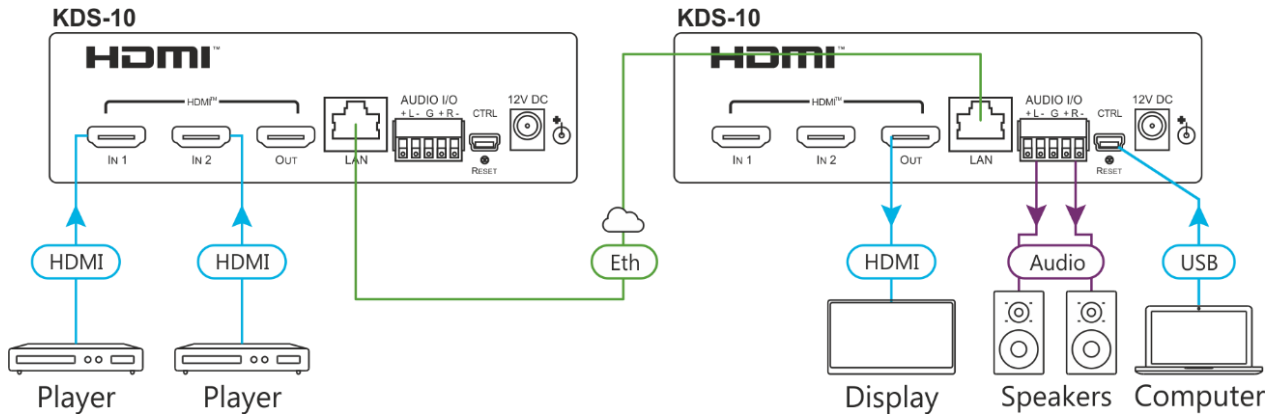
Figure 2: Connecting to the KDS-10 Rear Panel
