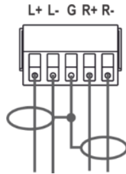
Figure 3: Connecting to a Balanced Stereo Audio Acceptor
