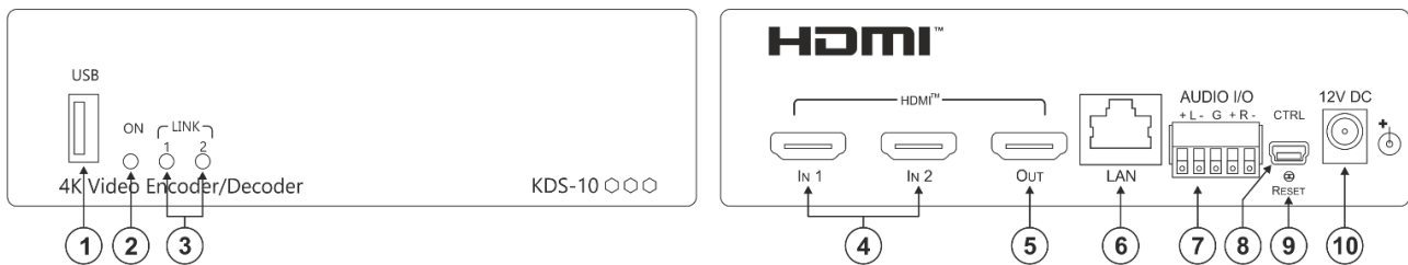
Figure 1: KDS-10 4K Video Encoder/Decoder front and back panel
