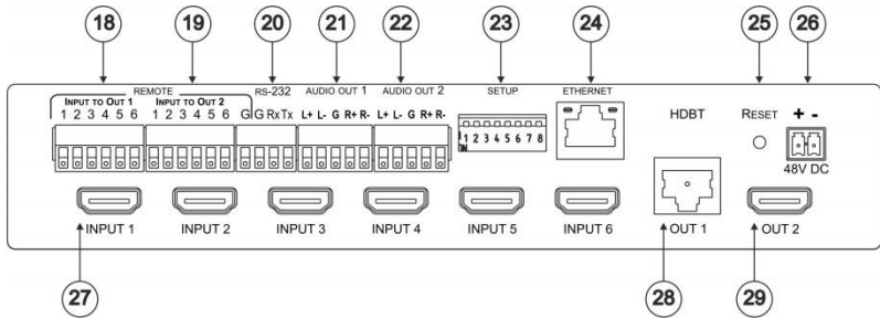
Figure 2: VS-62DT 6x2 UHD Matrix Switcher
