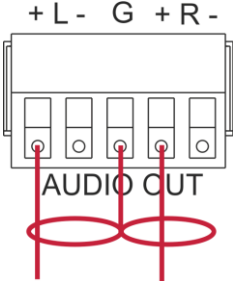
Figure 5: Connecting to an Unbalanced Stereo Audio Acceptor
